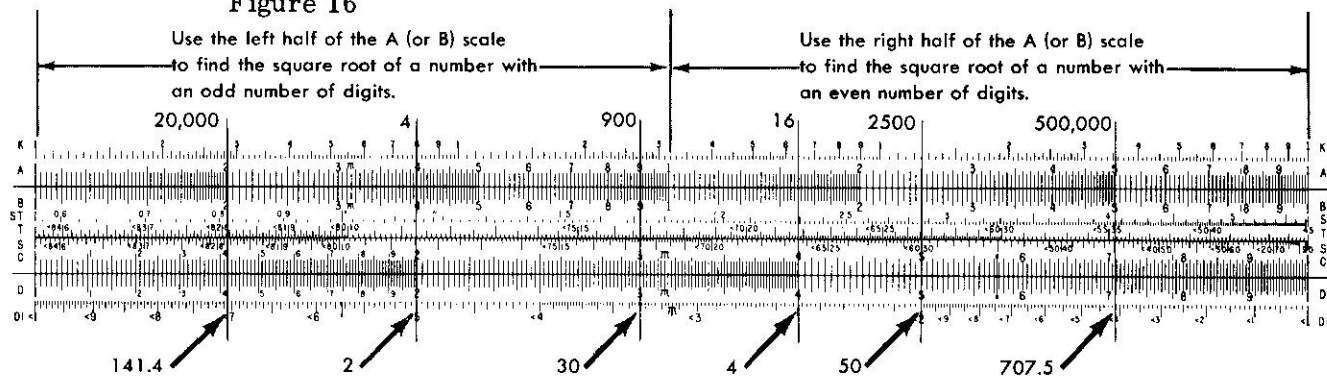
The square root of a number located on the A (or B) scale is found below on the D (or C) scale.
