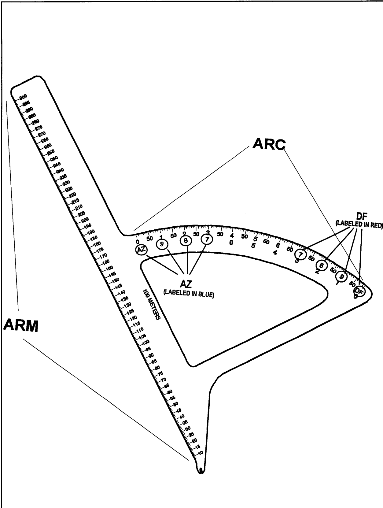
Figure 6-4. Range-Deflection Protractor.
