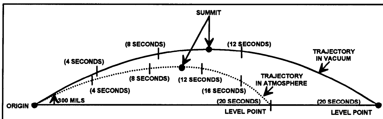
Figure 3-8. Trajectory in a Standard Atmosphere and in a Vacuum.
