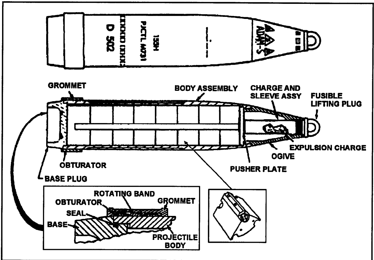
Figure 13-18. ADAM Projectile.
