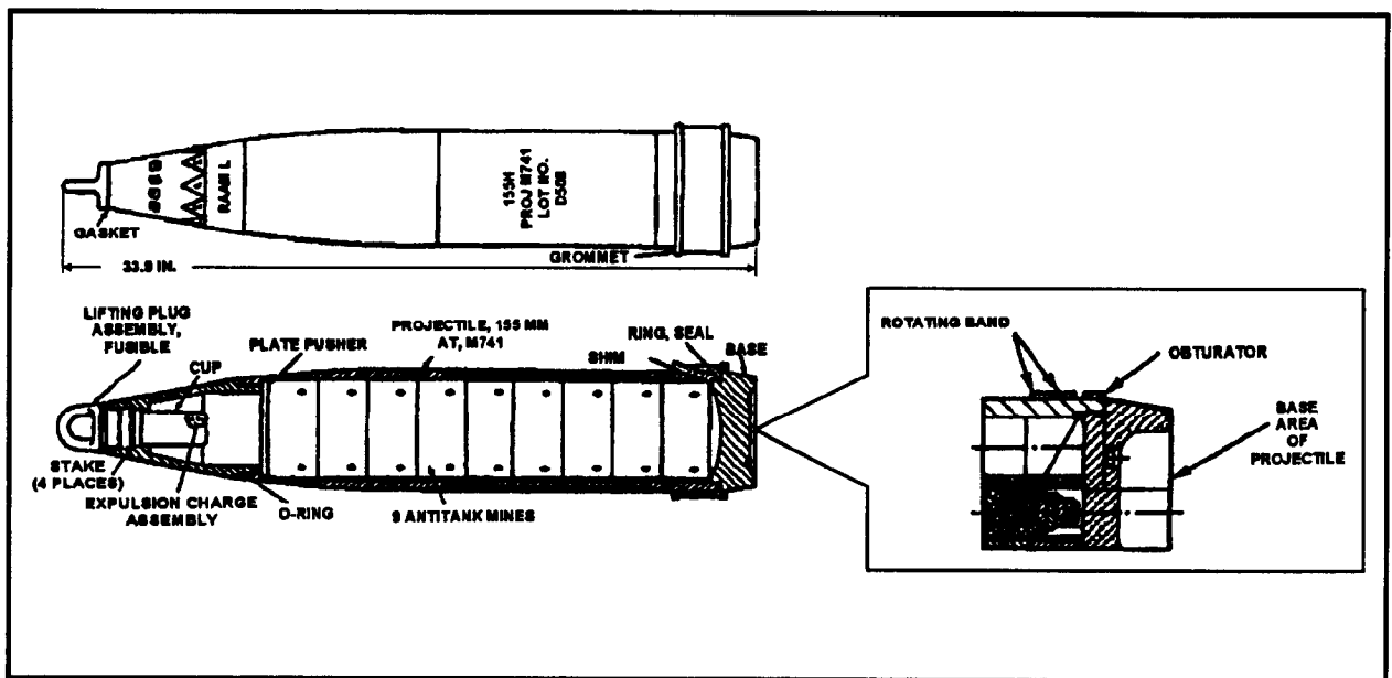
Figure 13-19. RAAMS Projectile.
