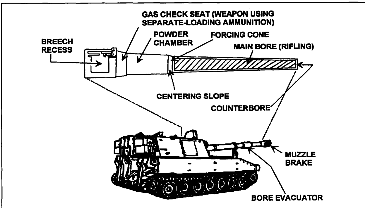
Figure 3-1. Cannon Tube.
