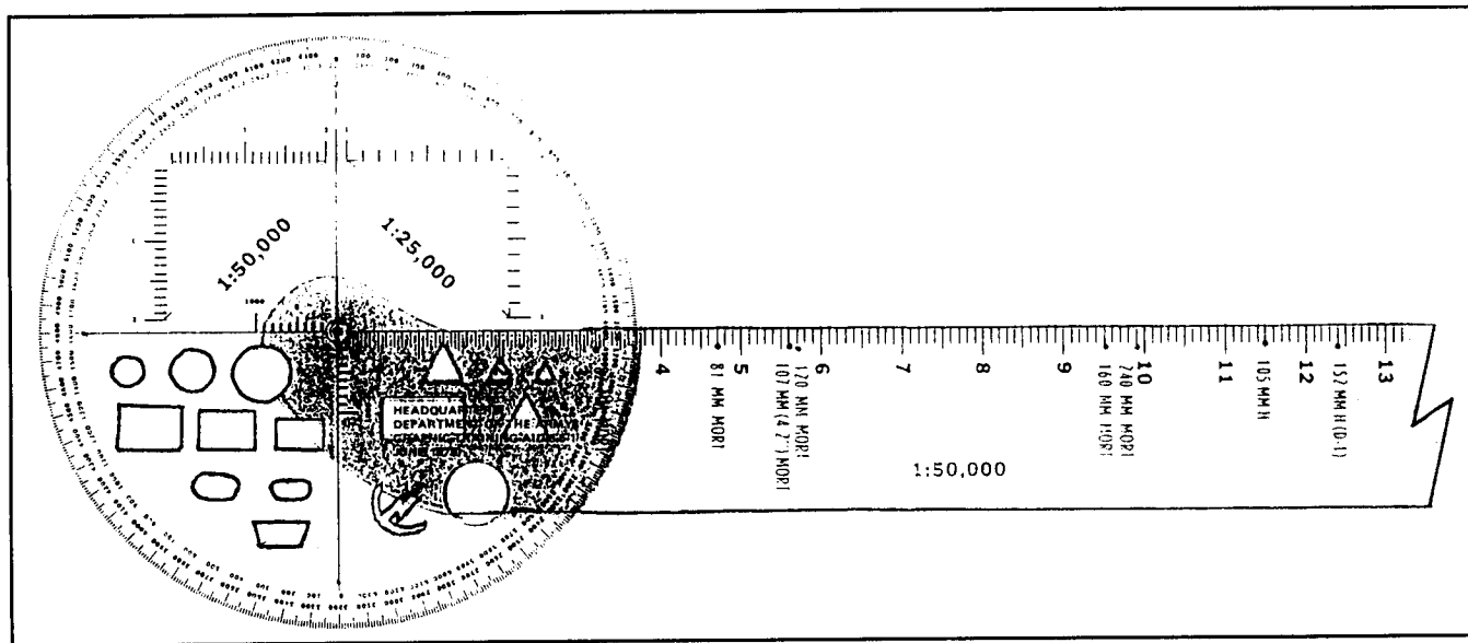
Figure 14-1. Range-Azimuth Fan.
