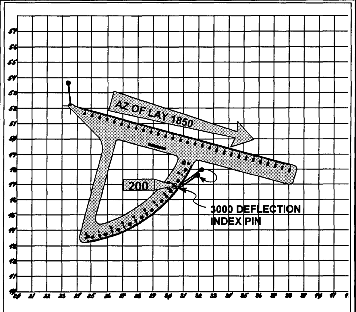
Figure 6-17. Common Deflection.
