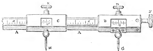
THE BEAM COMPASSES.
