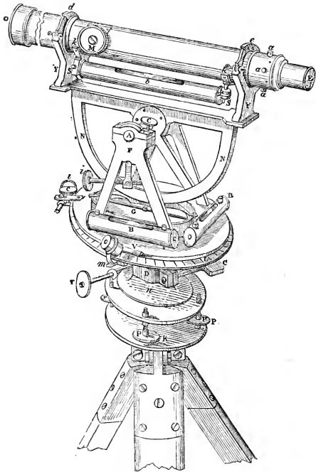
A Five-Inch Theodolite.
